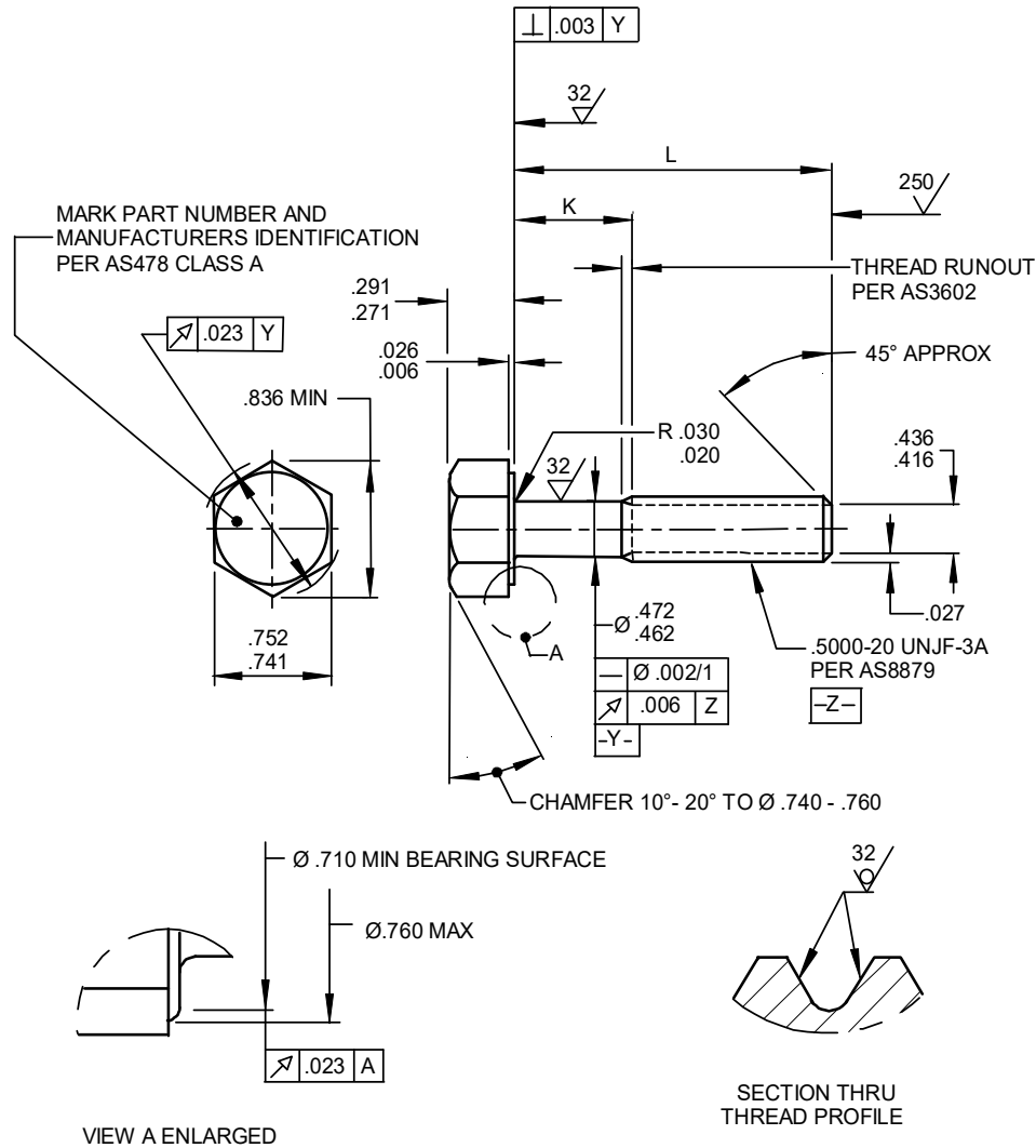
FIGURE 1 - BOLT
